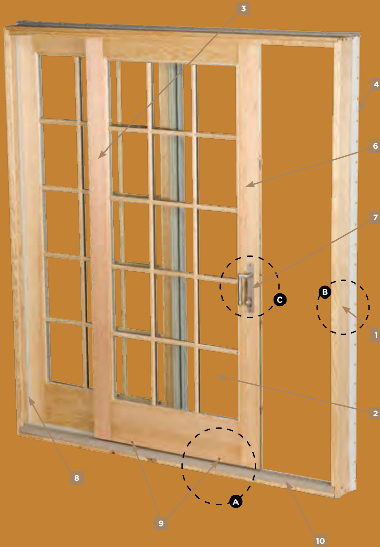
EXTERIOR DETAIL
