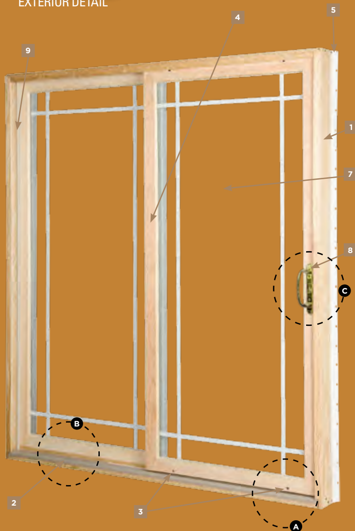
EXTERIOR DETAIL
